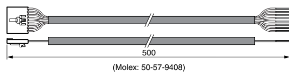
Figure 12: Dimensional Outline (Unit: mm)
