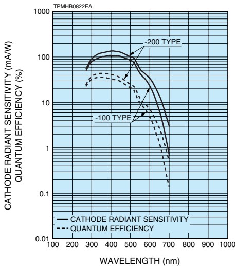
-100 and -200 Types
