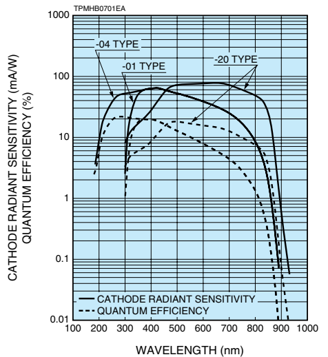
-01, -04 and -20 Types
