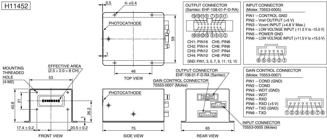
Figure 11: Dimensional Outline (Unit: mm)
