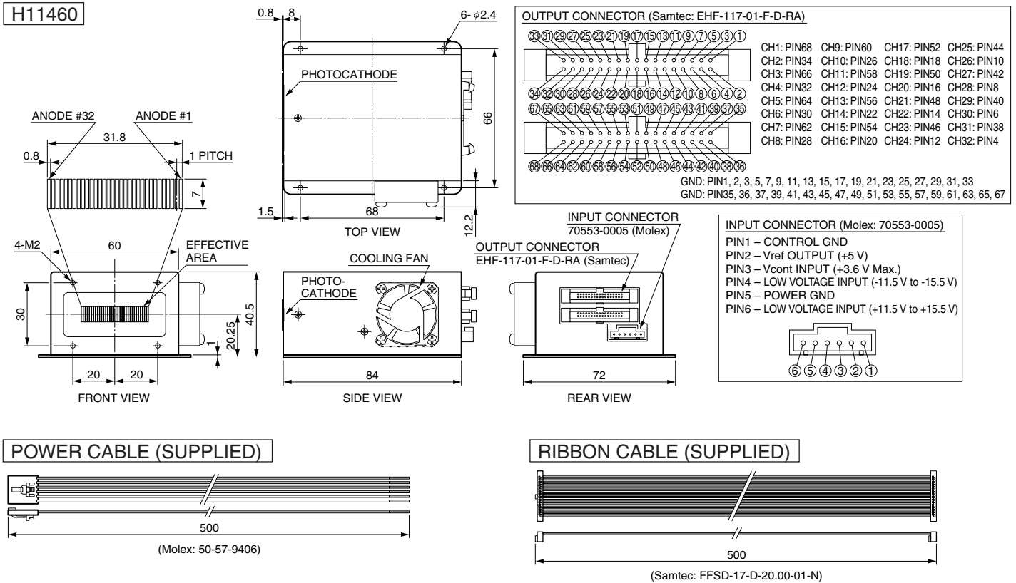
Figure 13: Dimensional Outline (Unit: mm)
