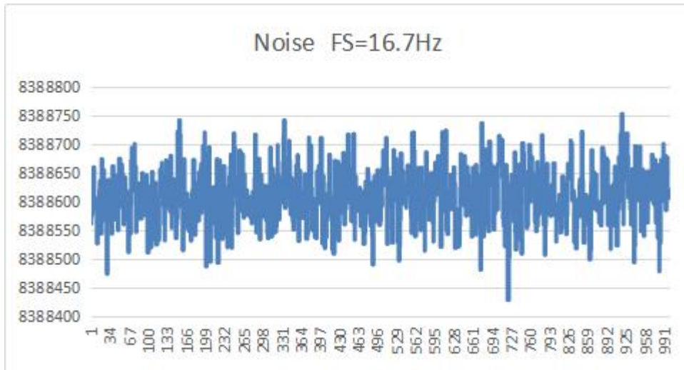
MS5197T 噪声 ( AVDD=4V,VREF = 2.048, Update Rate = 16.7 Hz )
