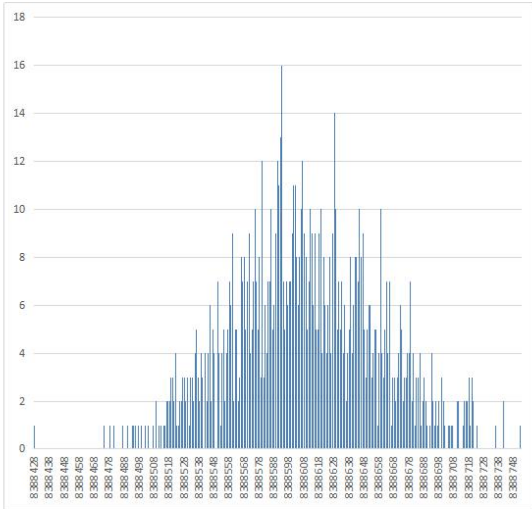
MS5196T 噪声分布柱状图 ( AVDD=4V,VREF = 2.048, Update Rate = 16.7 Hz )
