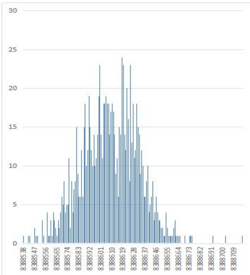
MS5197T 噪声分布柱状图 ( AVDD=4V,VREF = 2.048, Update Rate = 4.17 Hz )
