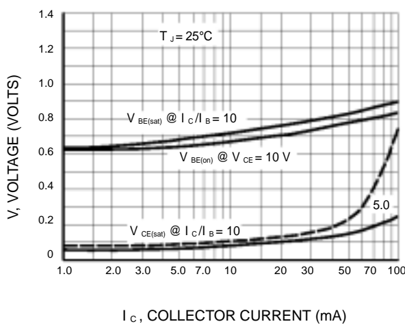
Figure 4. "On" Voltages
