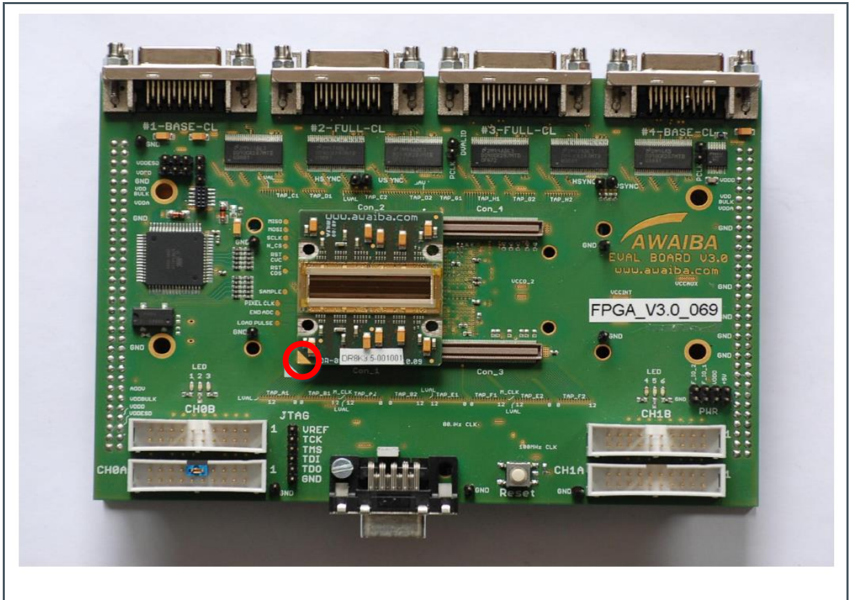
Figure 10: Assembling DR8K3.5 on the Evaluation Board
