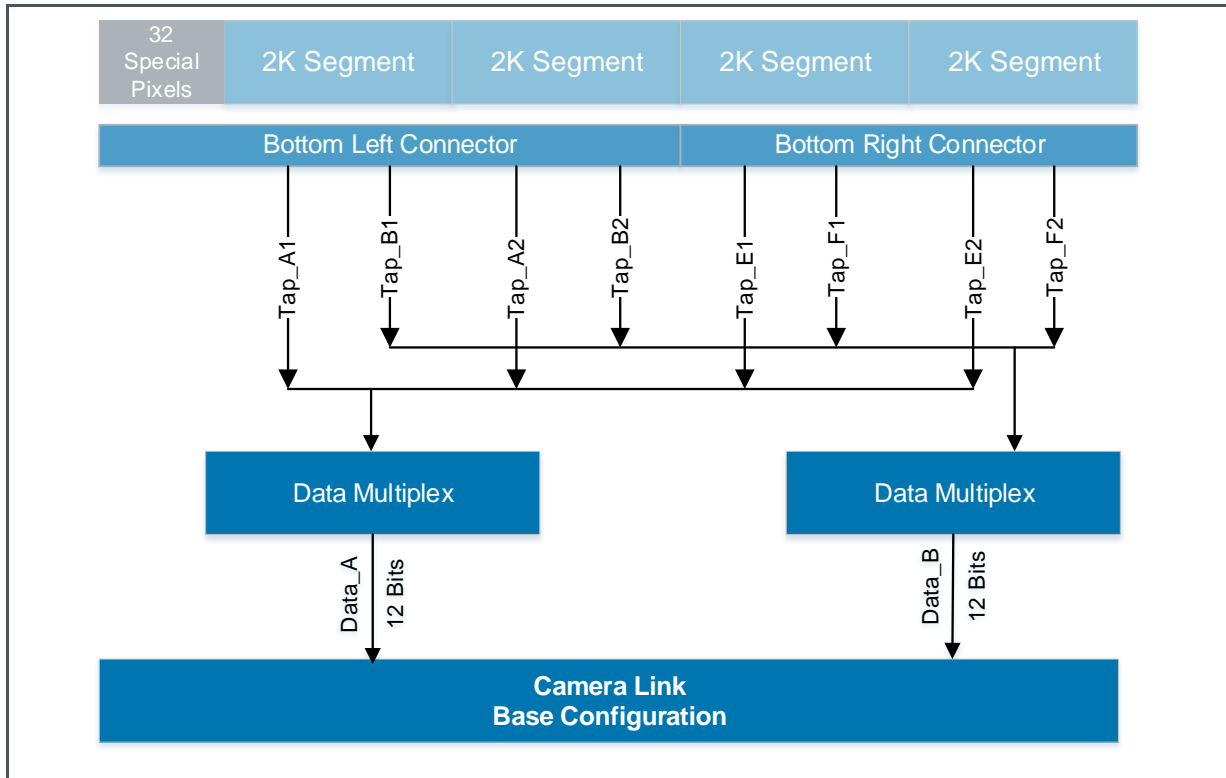
Figure 13: Camera-Link Output DR8K7um
