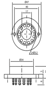
CR193-02A/03A 管座E678-12A
