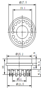
CR193-02/03 管座E678-14T
